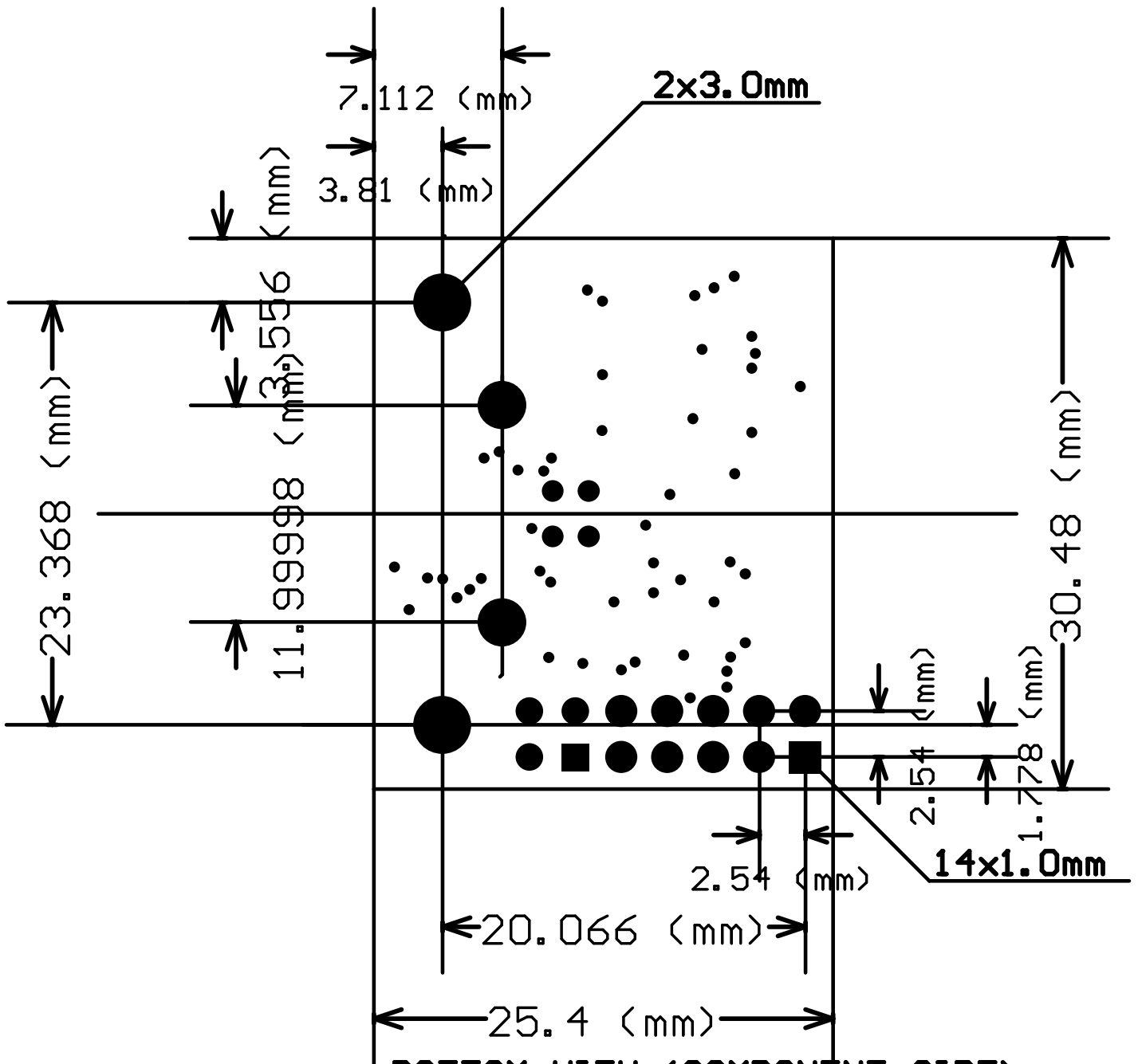
BOTTOM VIEW (COMPONENT SIDE)
