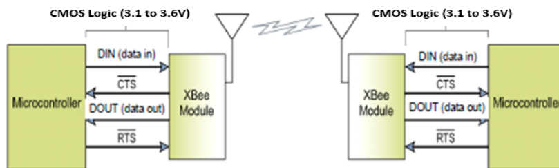
System Data Flow Diagram in a UART-interfaced environment (Low-asserted signals distinguished with horizontal line over signal name.)
