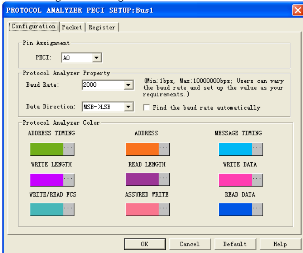
PECI Configuration dialog box
