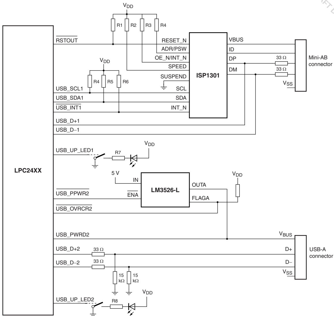
Fig 54. USB OTG port configuration: port U1 OTG Dual-Role device, port U2 host
