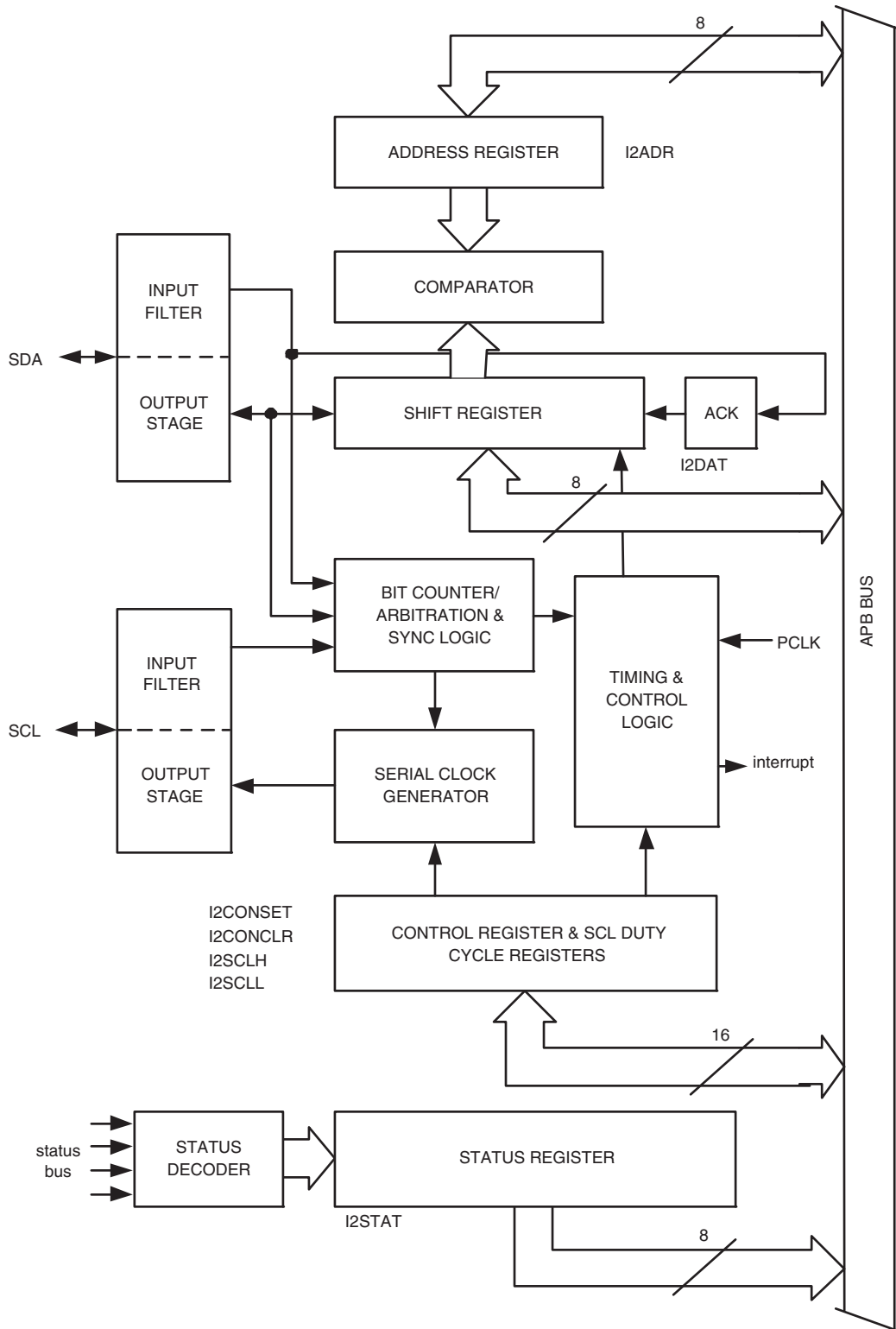
Fig 118. I 2 C Bus serial interface block diagram
