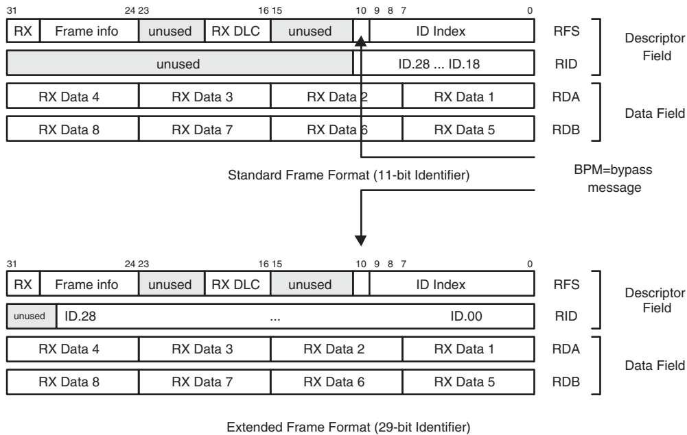
Fig 76. Receive buffer layout for standard and extended frame format configurations
