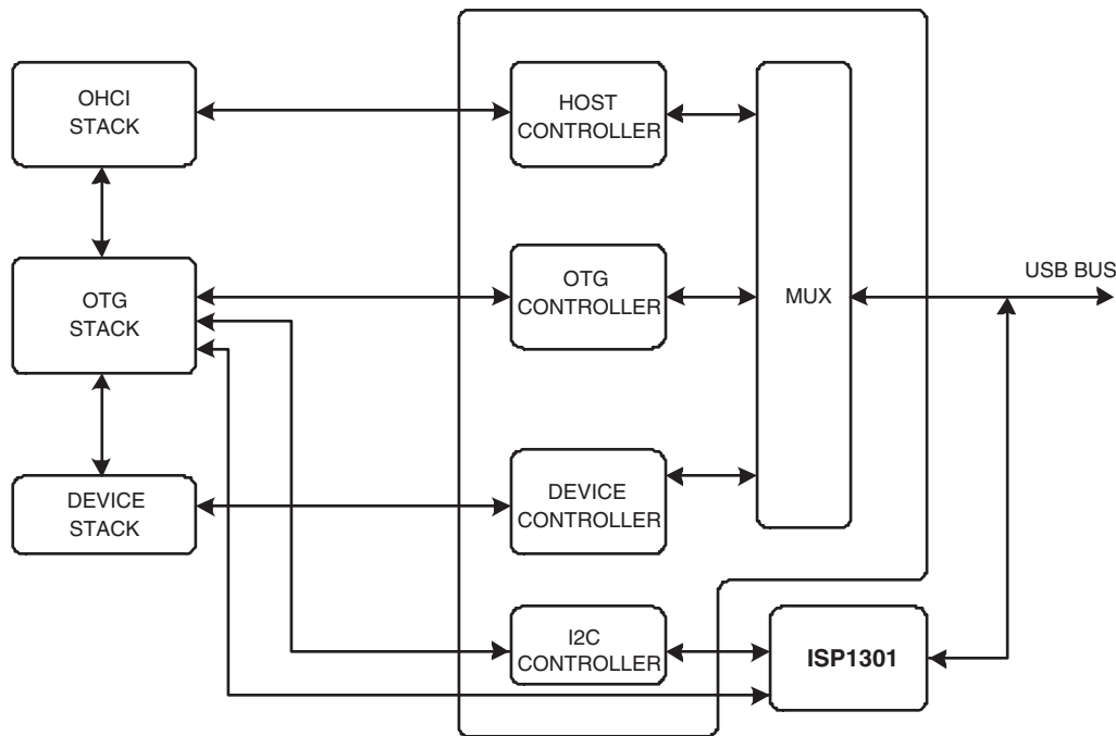
Fig 60. USB OTG controller with software stack
