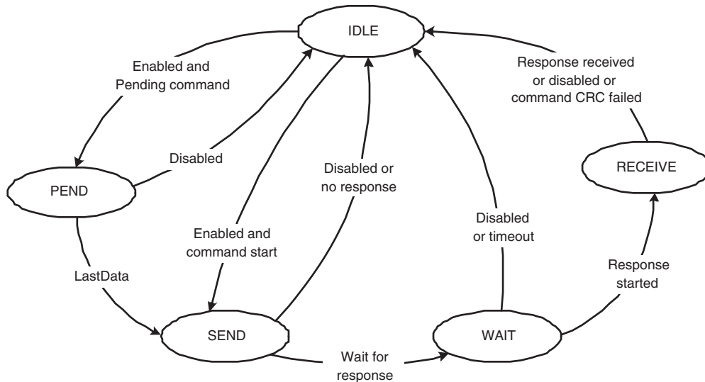
Fig 108. Command path state machine
