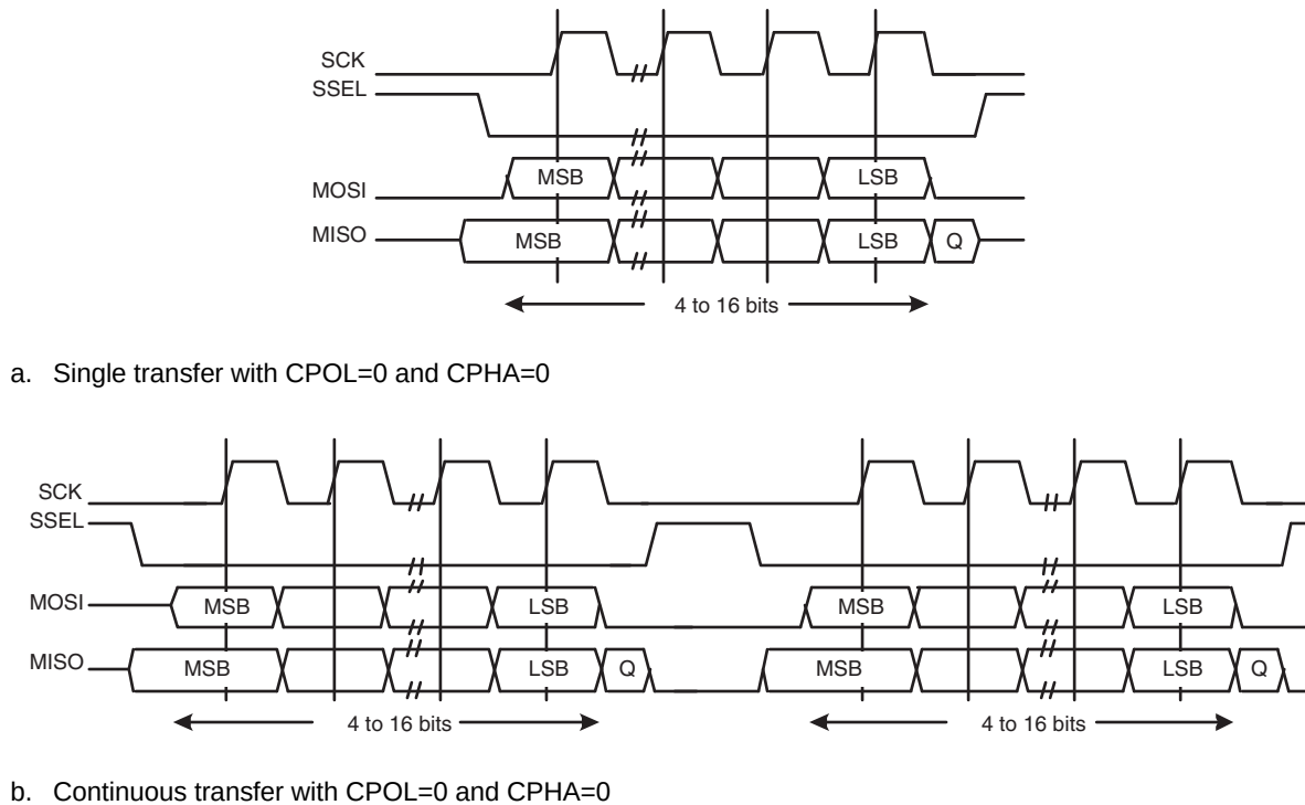
Fig 98. SPI frame format with CPOL=0 and CPHA=0 (a) Single and b) Continuous Transfer)
