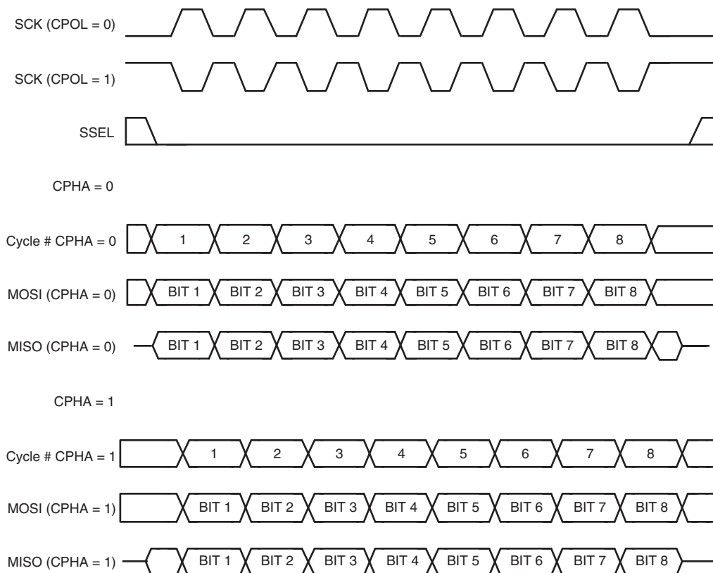
Fig 95. SPI data transfer format (CPHA = 0 and CPHA = 1)
