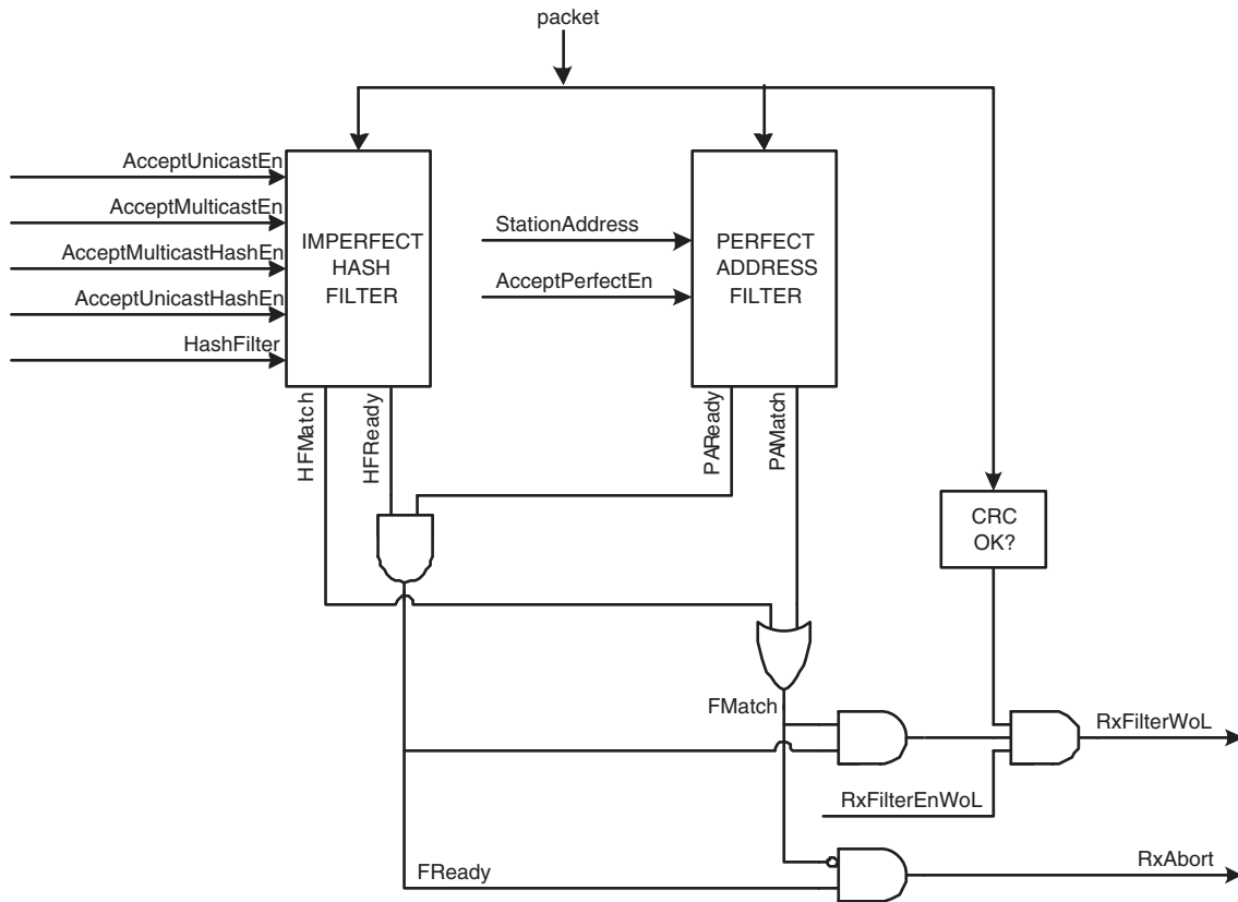
Fig 34. Receive filter block diagram
