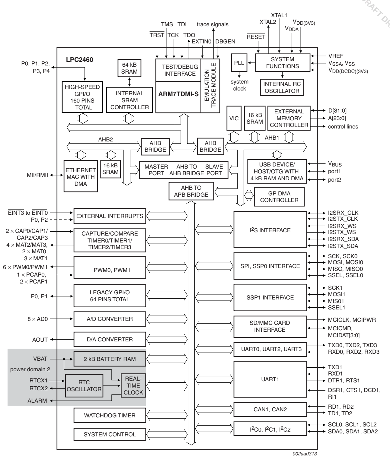
Fig 2. LPC2460 block diagram
