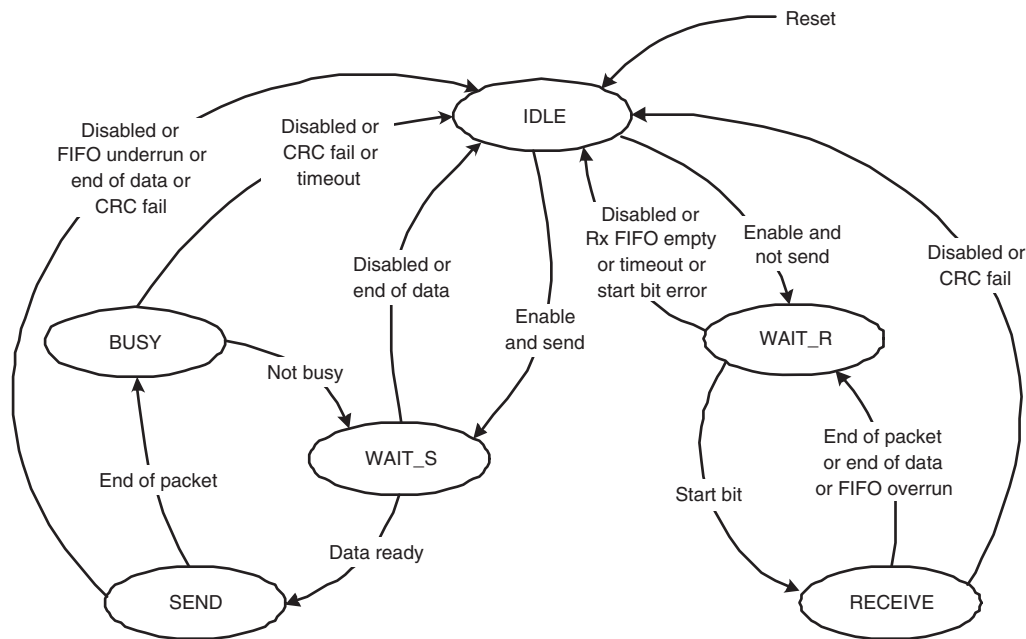
Fig 110. Data path state machine
