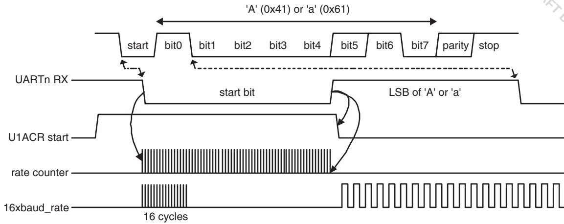
Fig 66. Autobaud a) mode 0 and b) mode 1 waveform
