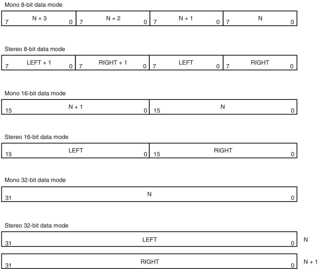
Fig 129.FIFO contents for various I 2 S modes
