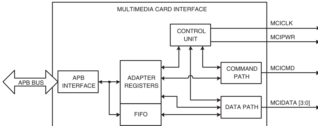
Fig 107.MCI adapter
