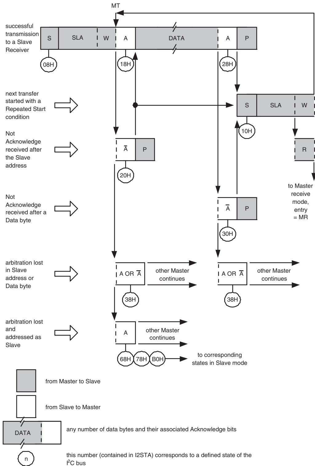
Fig 121.Format and States in the Master Transmitter mode
