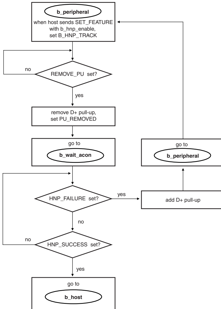
Fig 62. State transitions implemented in software during B-device switching from peripheral to host
