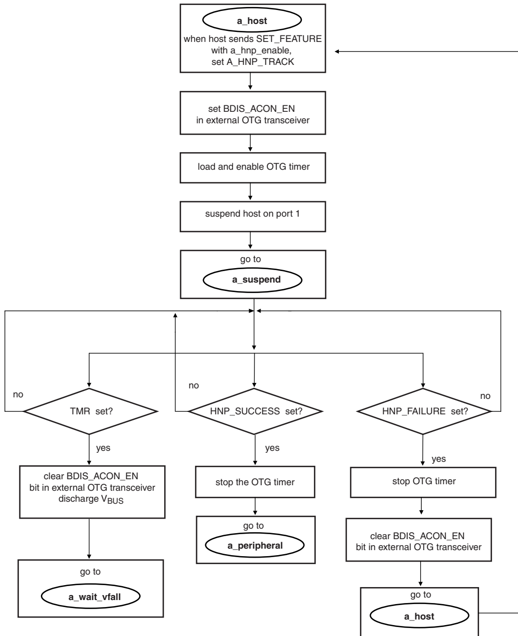
Fig 64. State transitions implemented in software during A-device switching from host to peripheral
