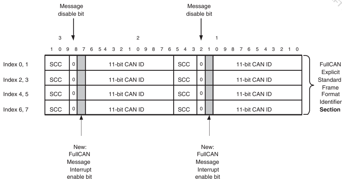
Fig 84. FullCAN section example of the ID look-up table
