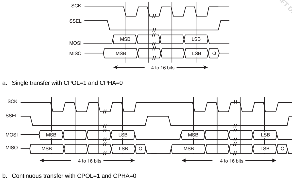
Fig 100. SPI frame format with CPOL = 1 and CPHA = 0 (a) Single and b) Continuous Transfer)
