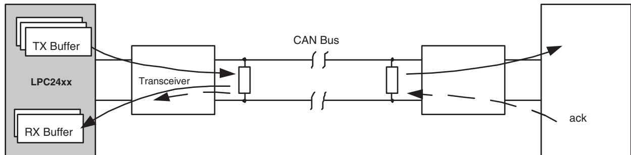
Fig 77. Global Self-Test (high-speed CAN Bus example)
