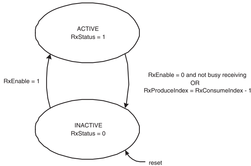
Fig 35. Receive Active/Inactive state machine
