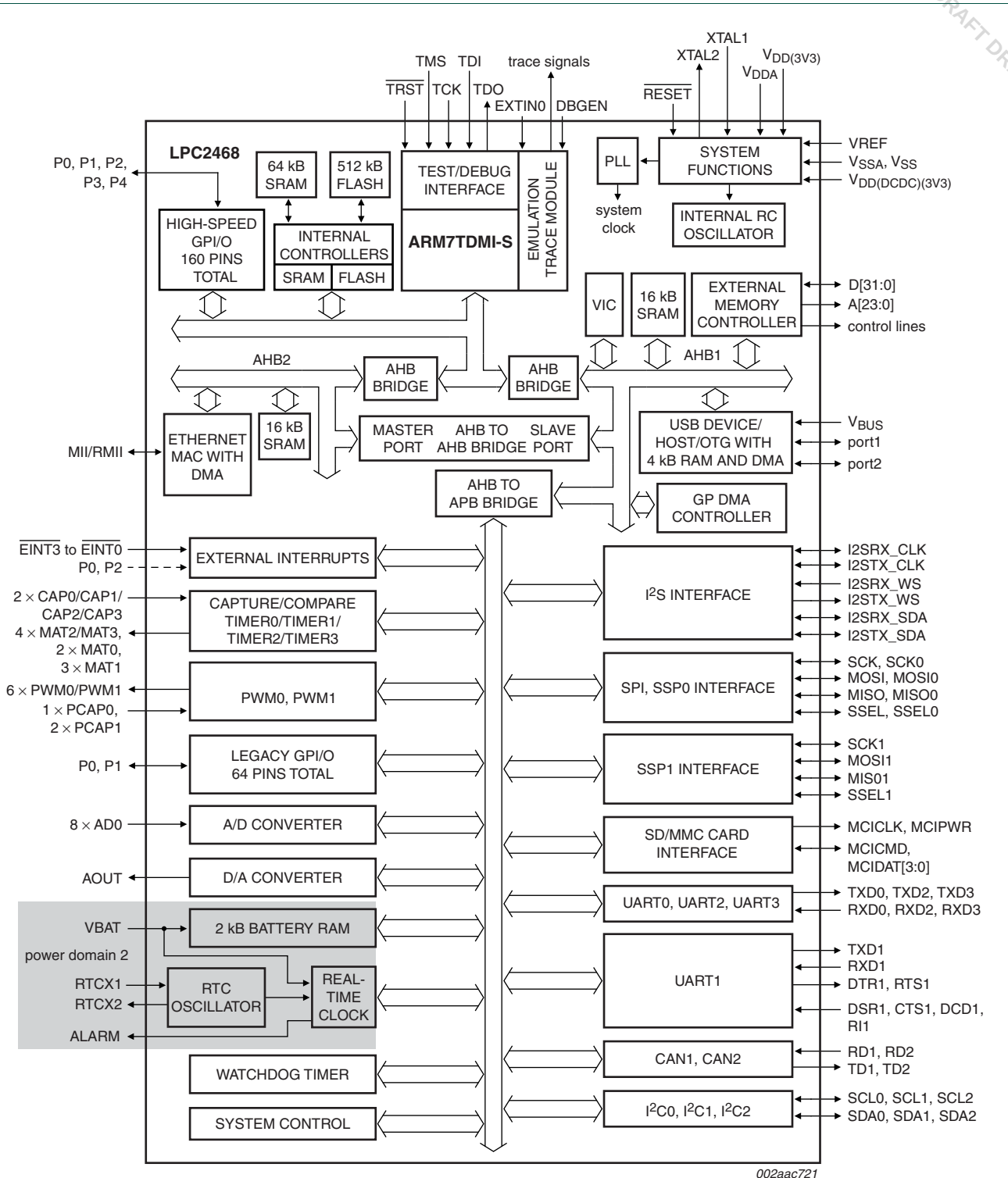
Fig 3. LPC2468 block diagram
