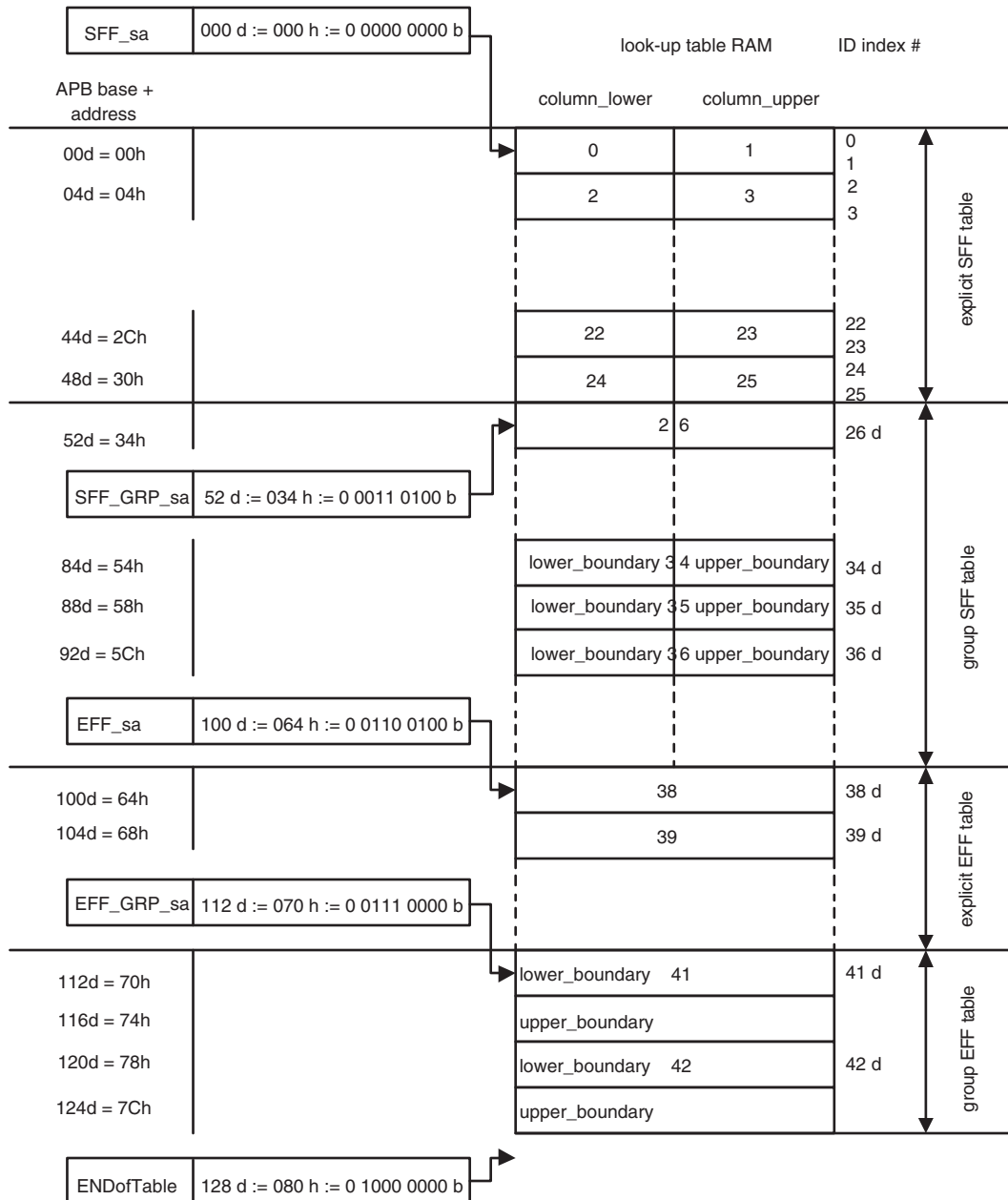
Fig 92. Detailed example of acceptance filter tables and ID index values
