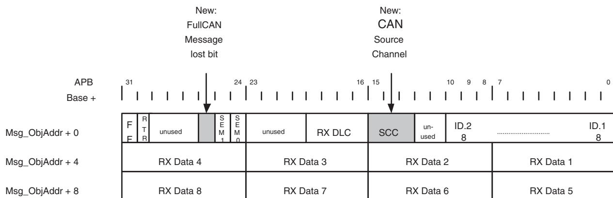
Fig 85. FullCAN message object layout
