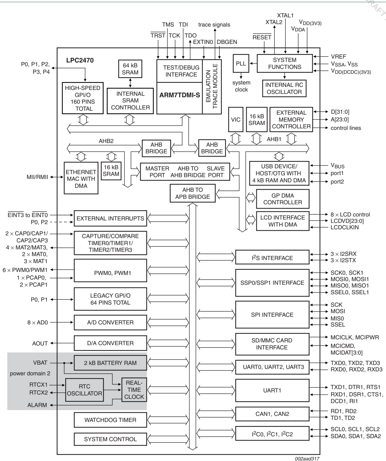
Fig 4. LPC2470 block diagram
