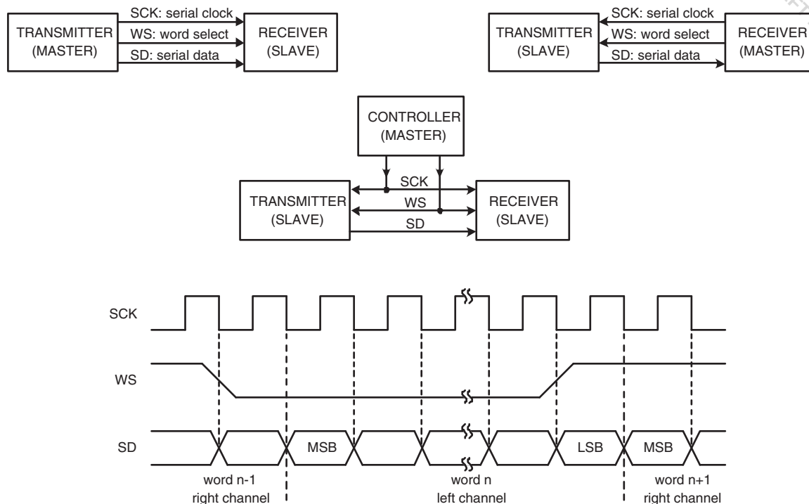
Fig 128. Simple I 2 S configurations and bus timing
