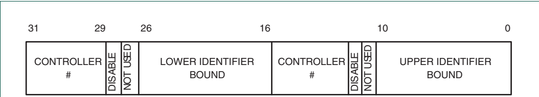
Fig 80. Entry in standard identifier range table
