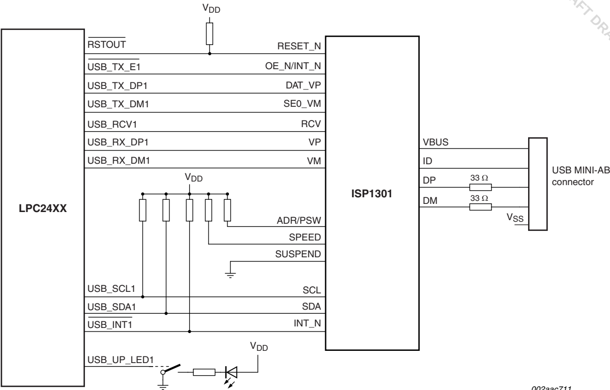
Fig 55. USB OTG port configuration: VP_VM mode
