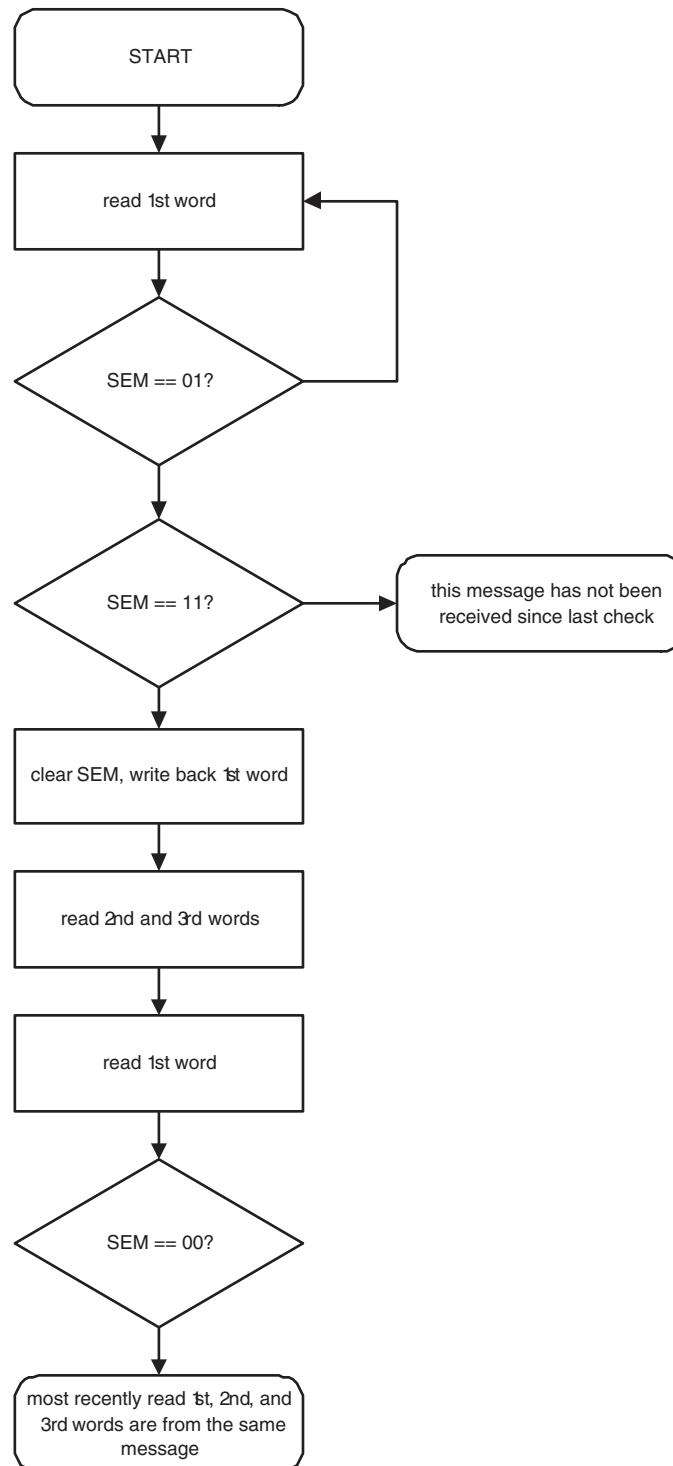
Fig 83. Semaphore procedure for reading an auto-stored message
