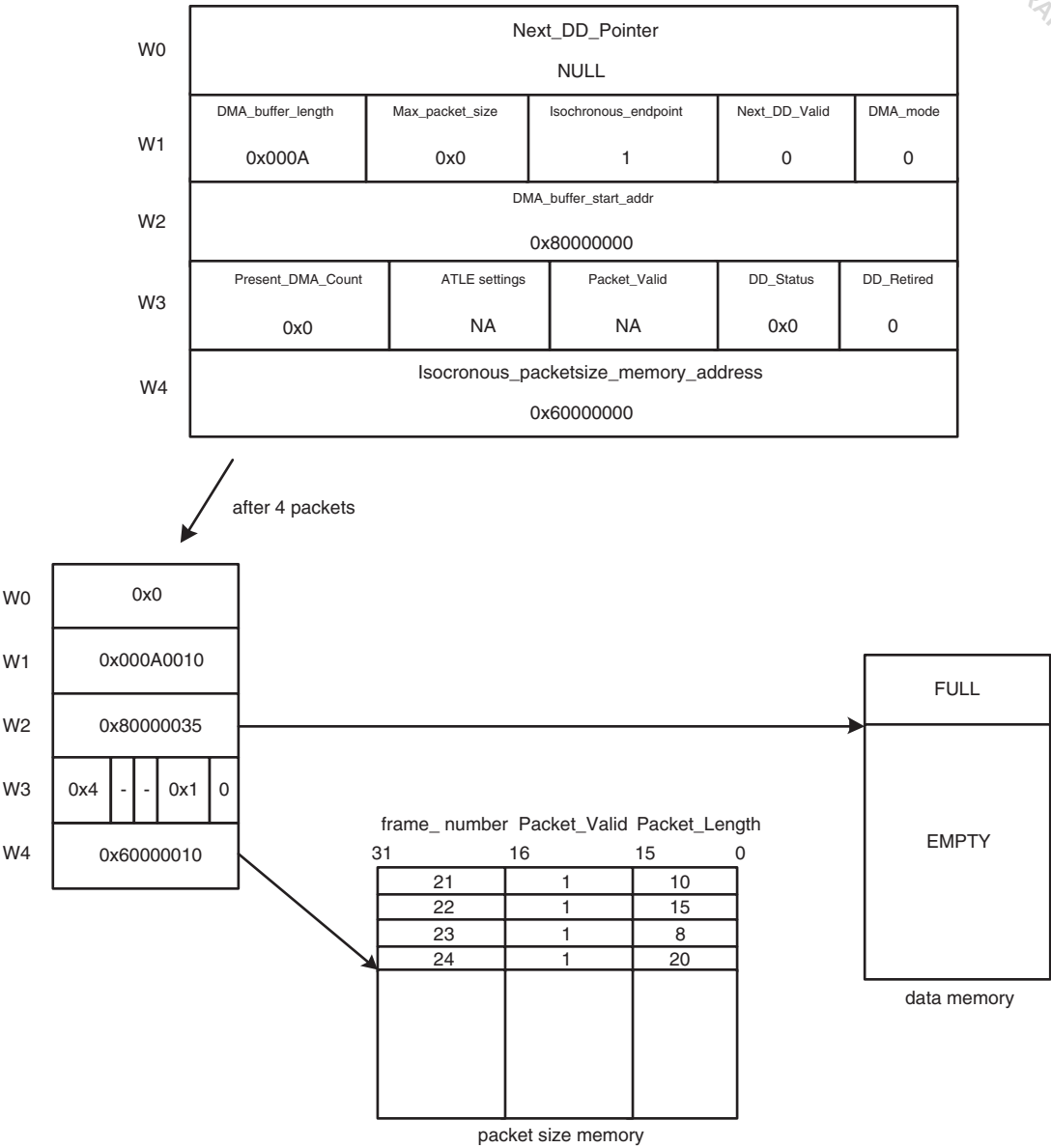
Fig 50. Isochronous OUT endpoint operation example
