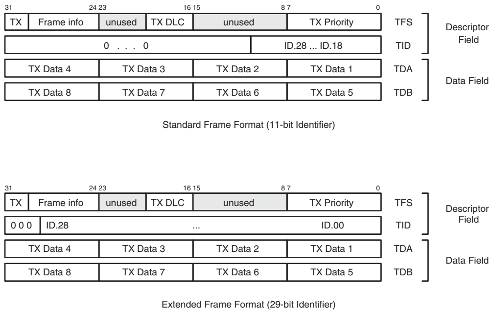
Fig 75. Transmit buffer layout for standard and extended frame format configurations
