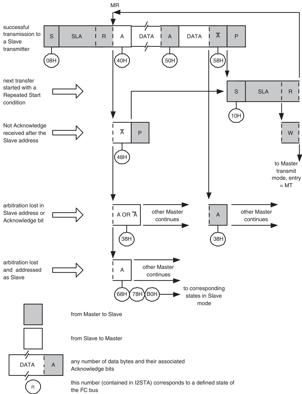
Fig 122.Format and States in the Master Receiver mode
