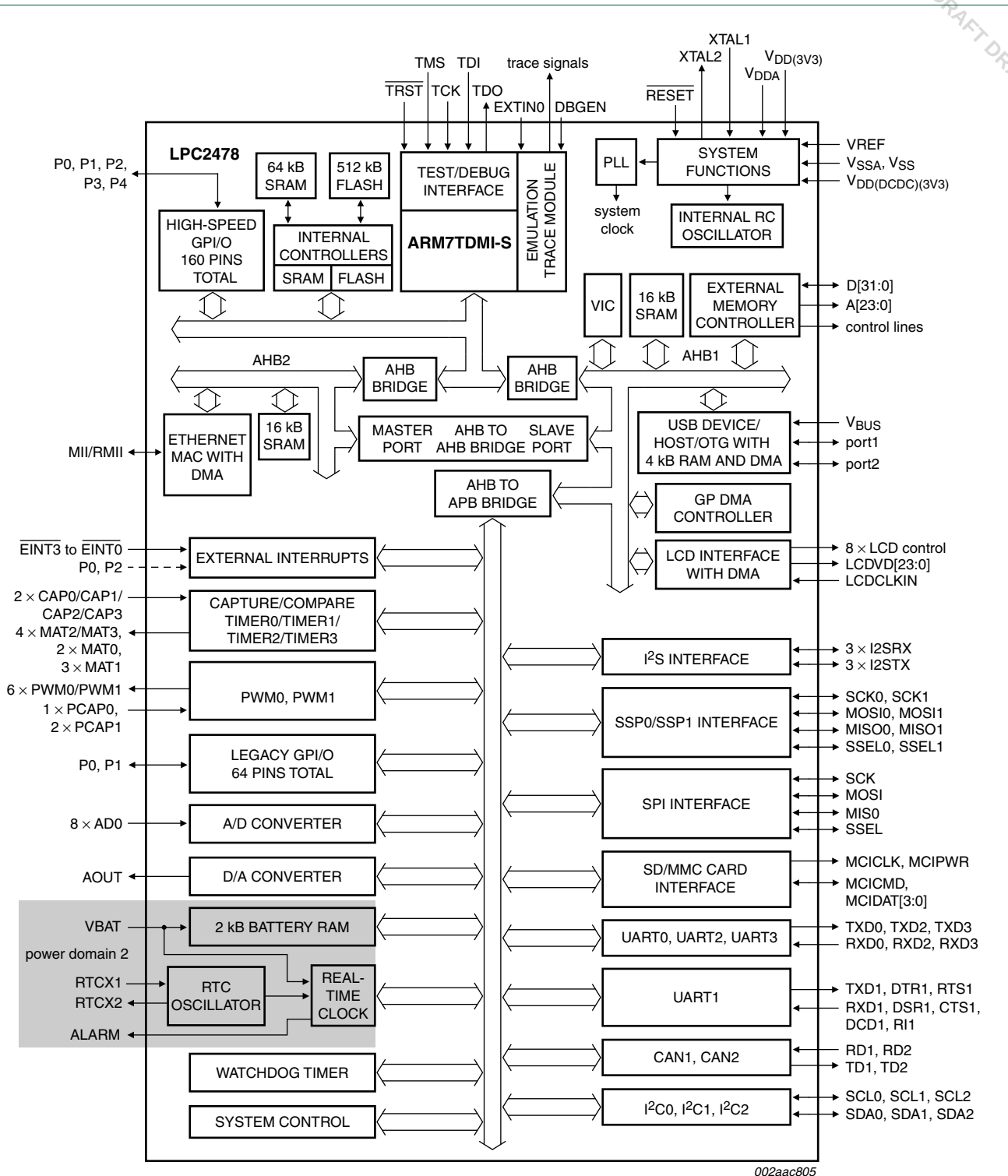
Fig 5. LPC2478 block diagram
