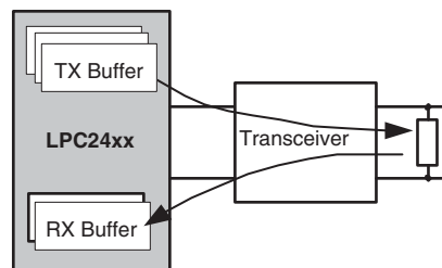
Fig 78. Local self test (high-speed CAN Bus example)
