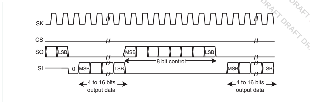
Fig 103.Microwire frame format (continuous transfers)
