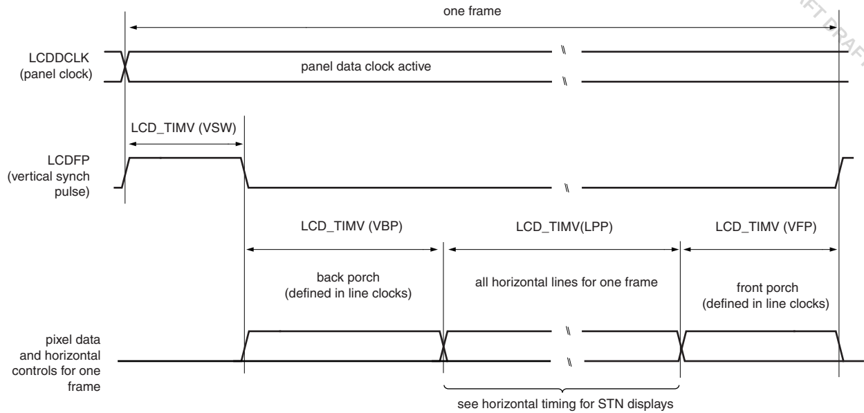
Fig 43. Vertical timing for STN displays
