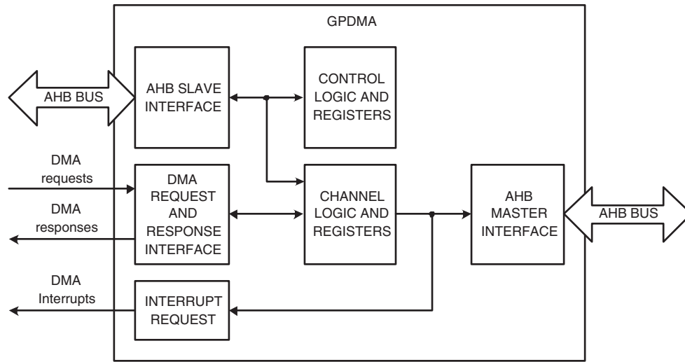
Fig 145.GPDMA block diagram
