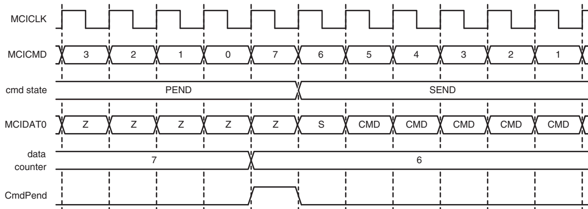
Fig 111. Pending command start
