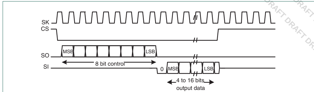
Fig 102. Microwire frame format (single transfer)
