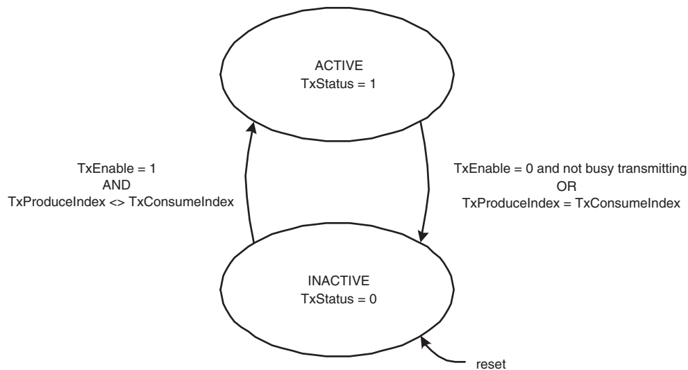
Fig 36. Transmit Active/Inactive state machine
