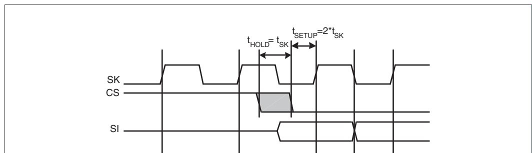
Fig 104.Microwire frame format setup and hold details
