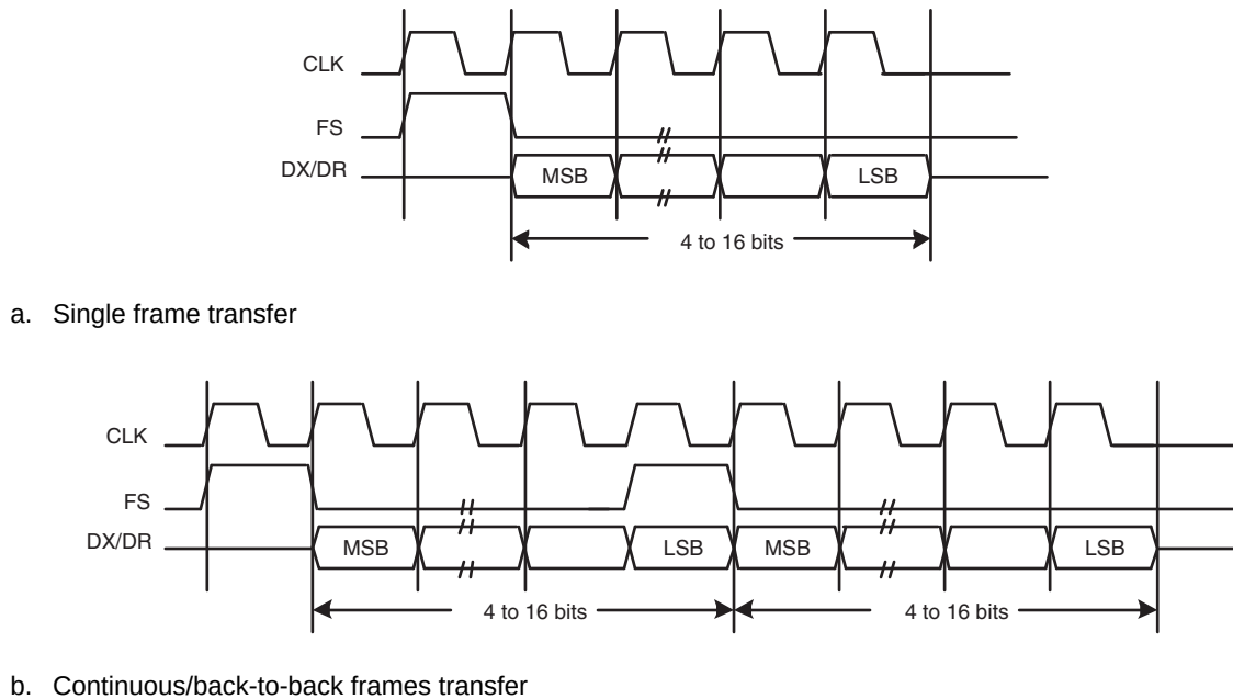
Fig 97. Texas Instruments Synchronous Serial Frame Format: a) Single and b) Continuous/back-to-back Two Frames Transfer
