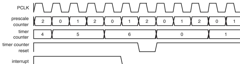
Fig 130.A timer cycle in which PR=2, MRx=6, and both interrupt and reset on match are enabled.
