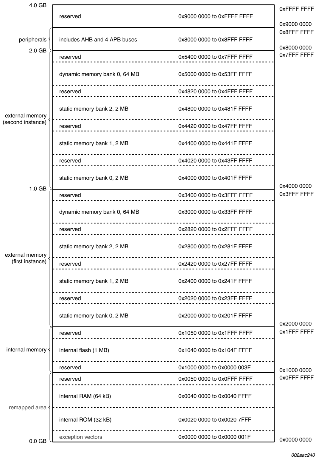
Fig 3. Memory map
