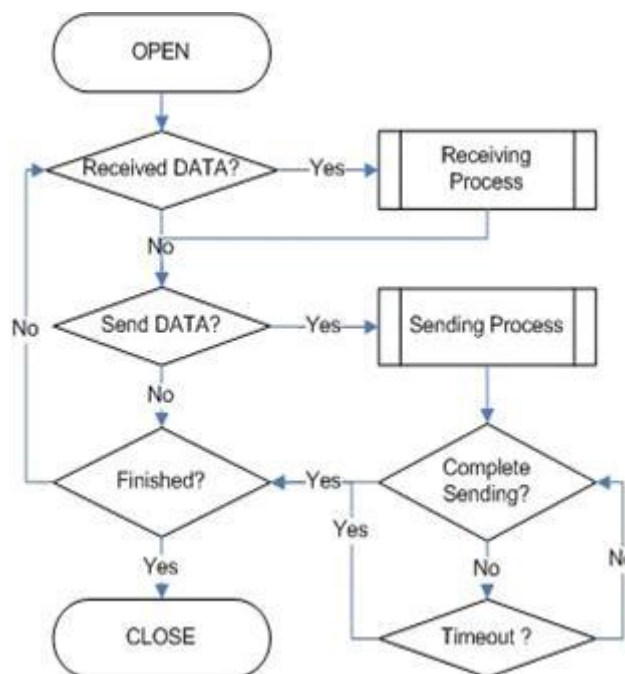
Figure 11 UDP Operation Flow
