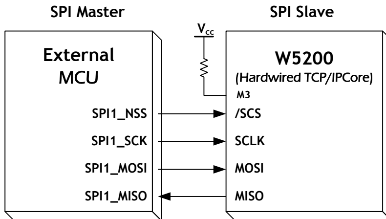
Figure 17 SPI Interface
