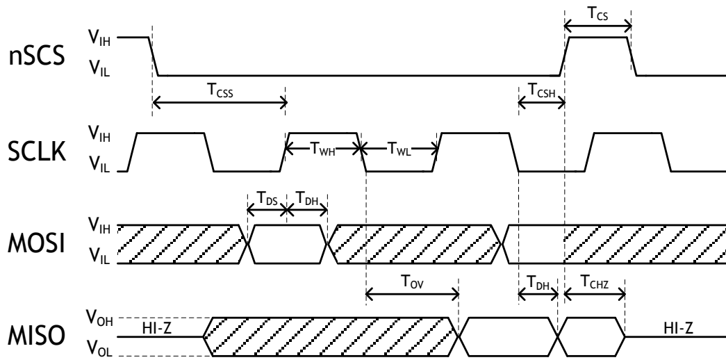
Figure 23 SPI Timing
