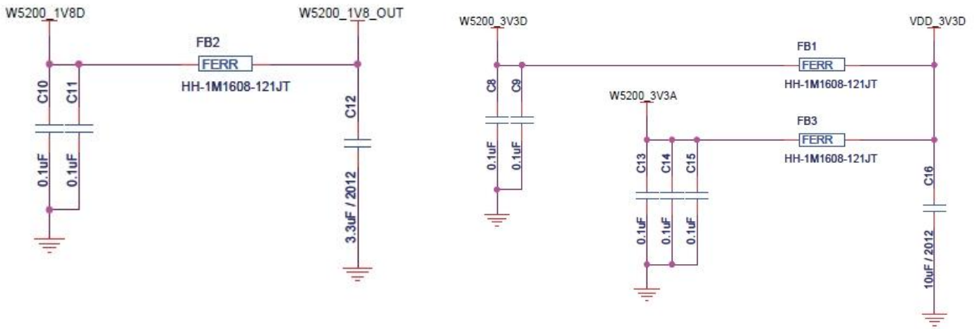
Figure 2 Power Design
