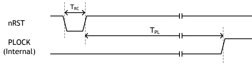
Figure 22 Reset Timing
