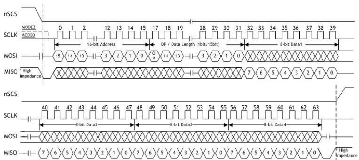
Figure 21 Write Sequence
