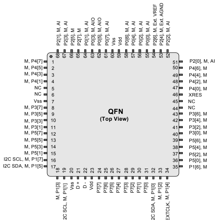
Figure 8-3. CY8C24994 68-Pin PSoC Device
