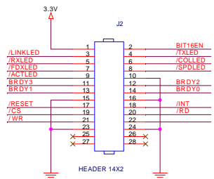
J1, J2 : 2.54mm pitch header
