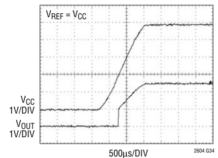
Power-On Reset to Midscale
