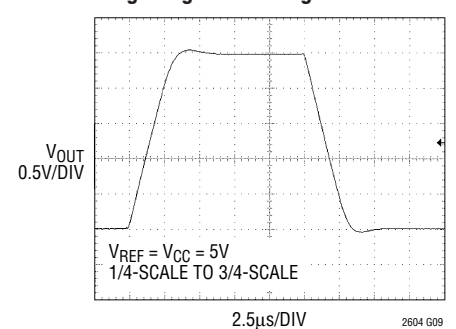
Large-Signal Settling
