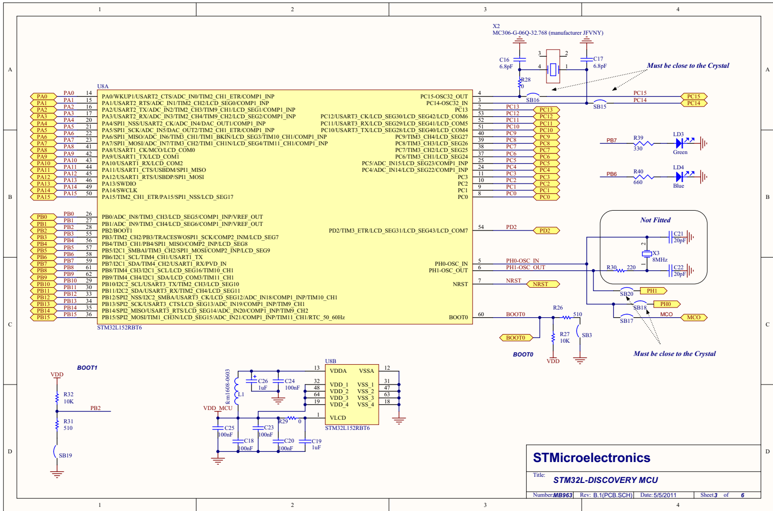
Figure 15. STM32L-DISCOVERY MCU
