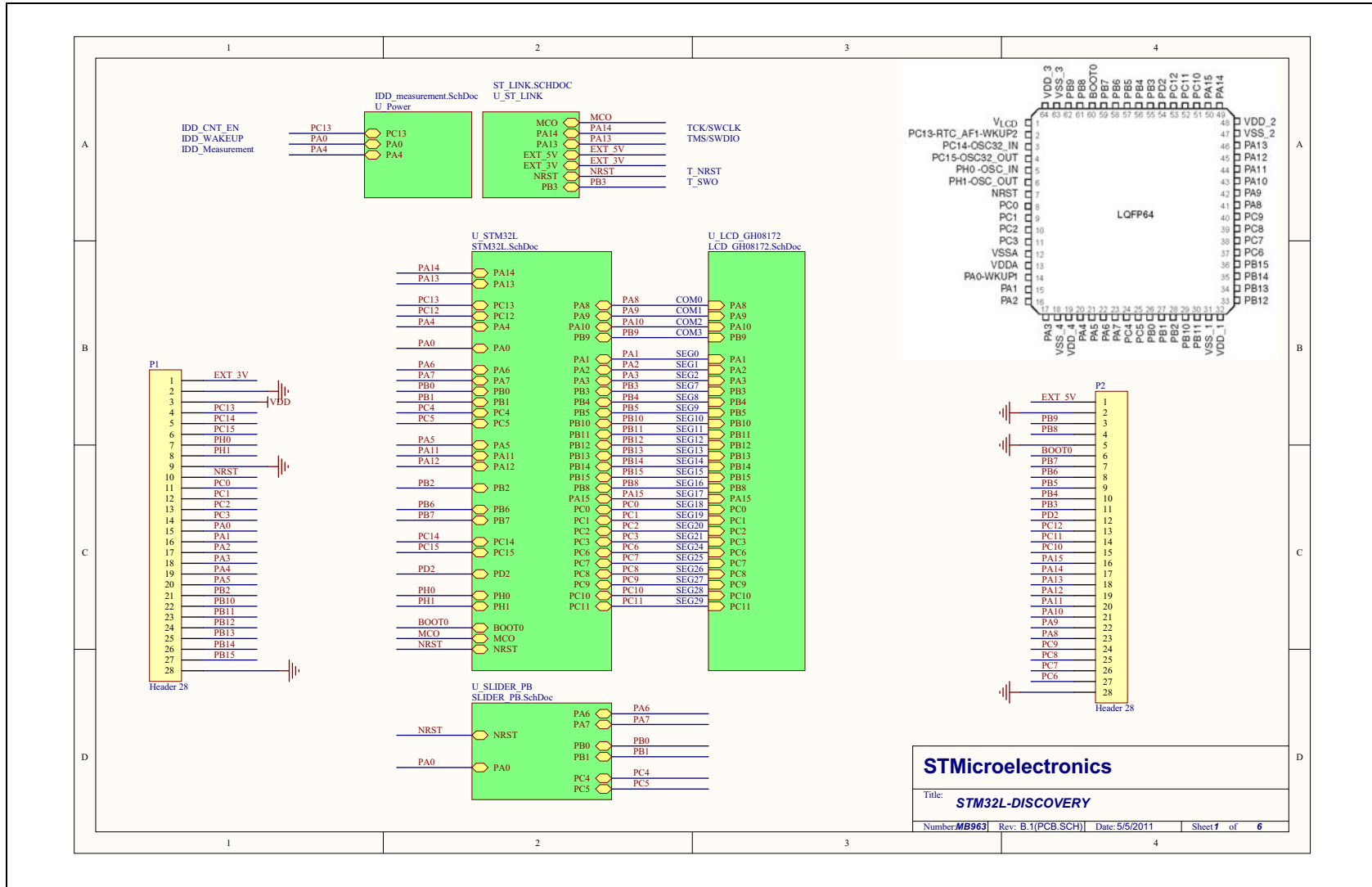
Figure 13. STM32L-DISCOVERY
