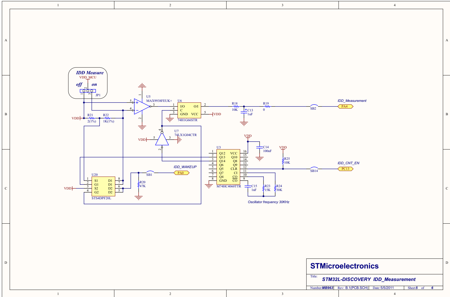
Figure 17. STM32L-DISCOVERY I DD measurement
