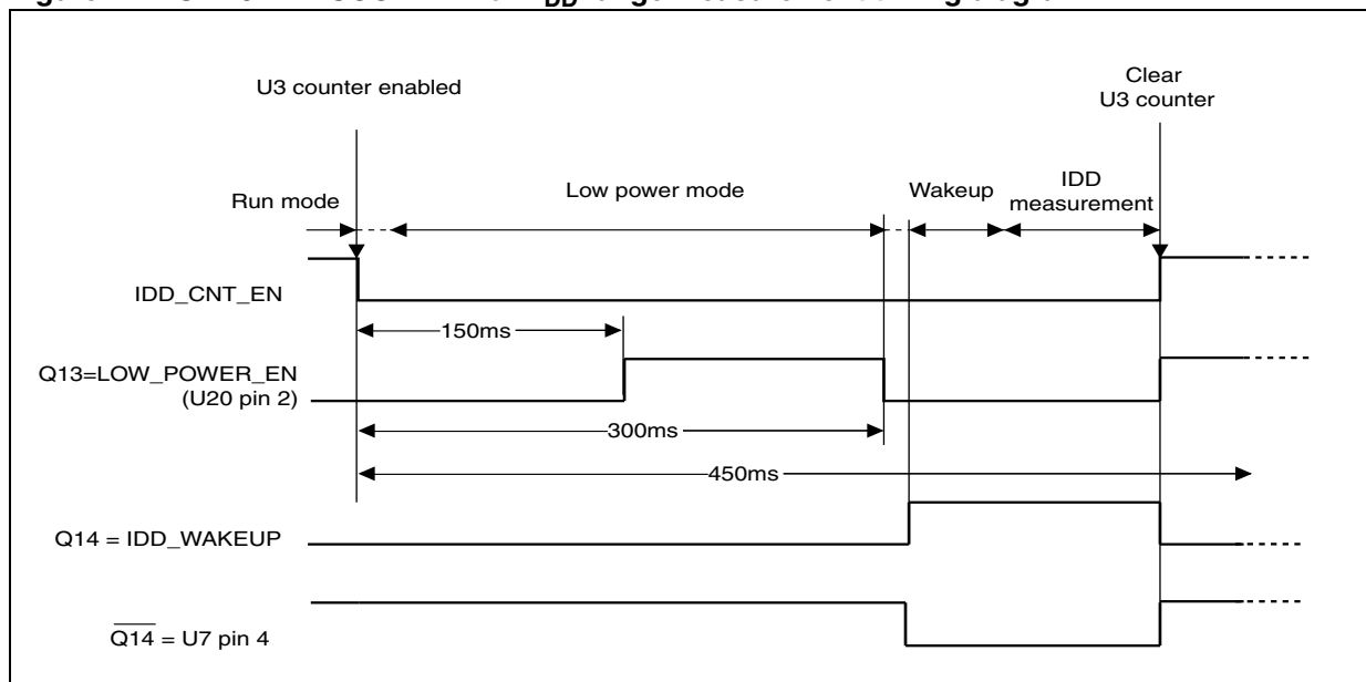
Figure 11. STM32L-DISCOVERY low I DD range measurement timing diagram
