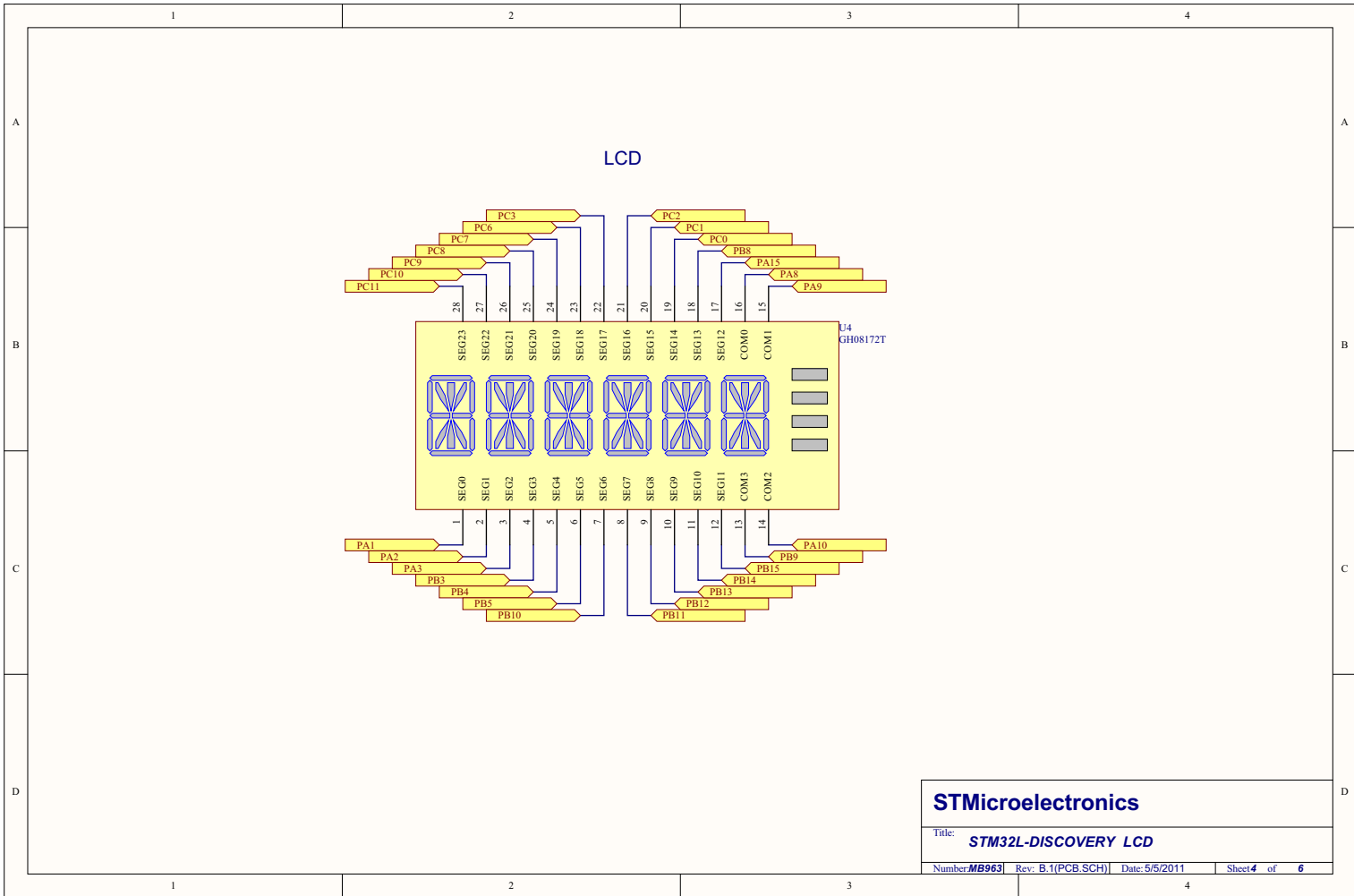
Figure 16. STM32L-DISCOVERY LCD
