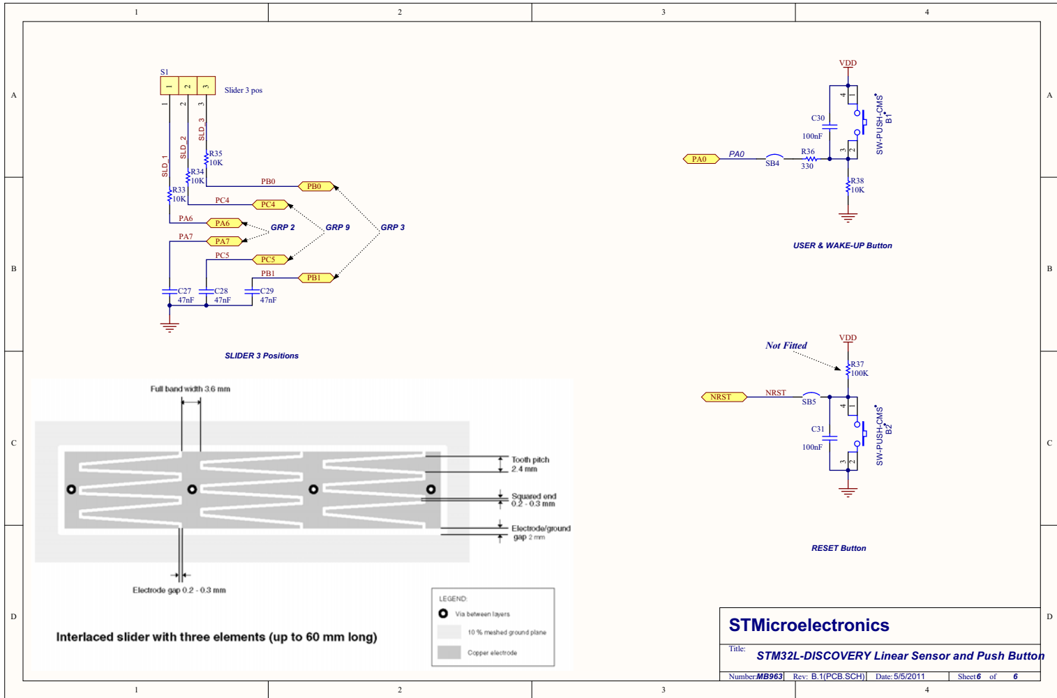
Figure 18. STM32L-DISCOVERY linear touch sensor/touchkeys
